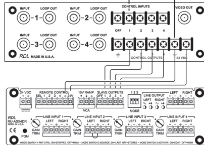
AUDIO FOLLOW VIDEO WIRING USING RDL RU-ASX4DR AUDIO SWITCHER
