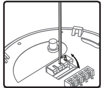
7b. Once aligned with central slot, pull cable up into slot to secure. Repeat steps 7a and 7b with secondary safety cable into one of the side slots.
