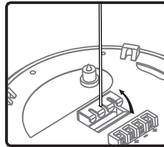
6. Align safety cable with center slot and pull up to secure.
