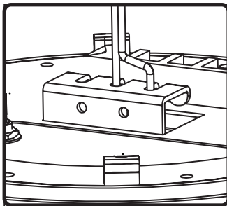
8. Extra slot and 2 holes provided for additional safety cables where needed.
