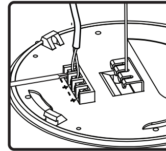
7. Connect signal wires to (+) and (-) inputs. Use extra (+) and (-) for daisy chaining.
