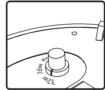
8. Select desired tap position. Switch is preset to maximum 70.7V (100V) mode.
