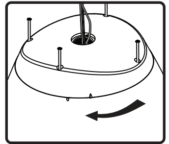
11. Place cover plate onto top of speaker and rotate clockwise until alignment indicators meet.
