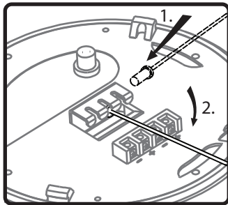
5. Attach safety cable by first inserting into side of mounting bracket.
