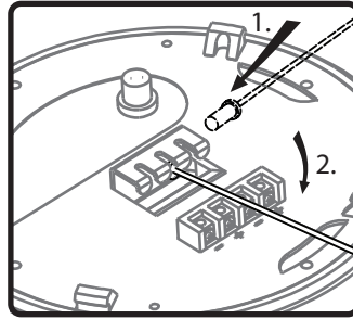
7a. Attach hanging cable by (1) inserting into side of mounting bracket and (2) rotating to align with center slot in hanging bracket.
