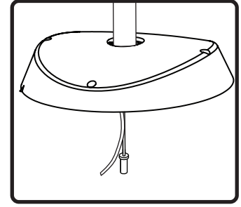
4. Run signal wire and at least one safety cable through conduit.
