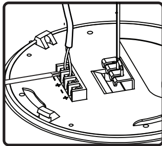
9. Connect signal wires to (+) and (-) inputs. Use extra (+) and (-) for daisy chaining.
