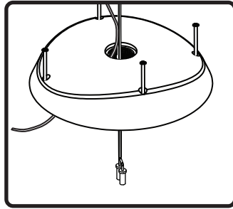
6. Slide cover plate over hanging and safety cables and run signal wire through center hole.
