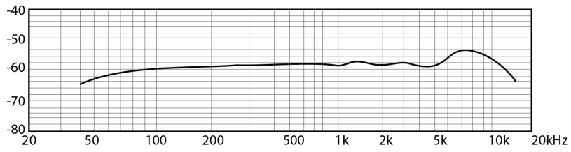
Frequency Response Graph
