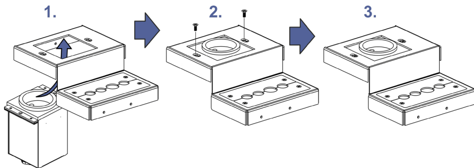
Figure 1: Power Socket Installation
