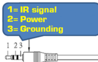
IR Receiver
