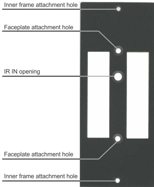
Figure 7: T-RC8IR (P/N: 80-000599)
