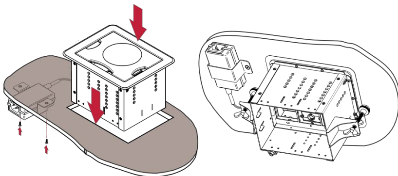
Figure 10: Inserting TBUS-1-KWC into the Prepared Opening
