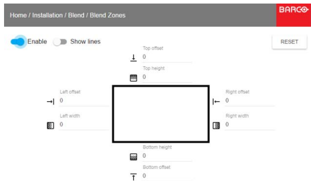
Image 8-24 Blend Zone menu
