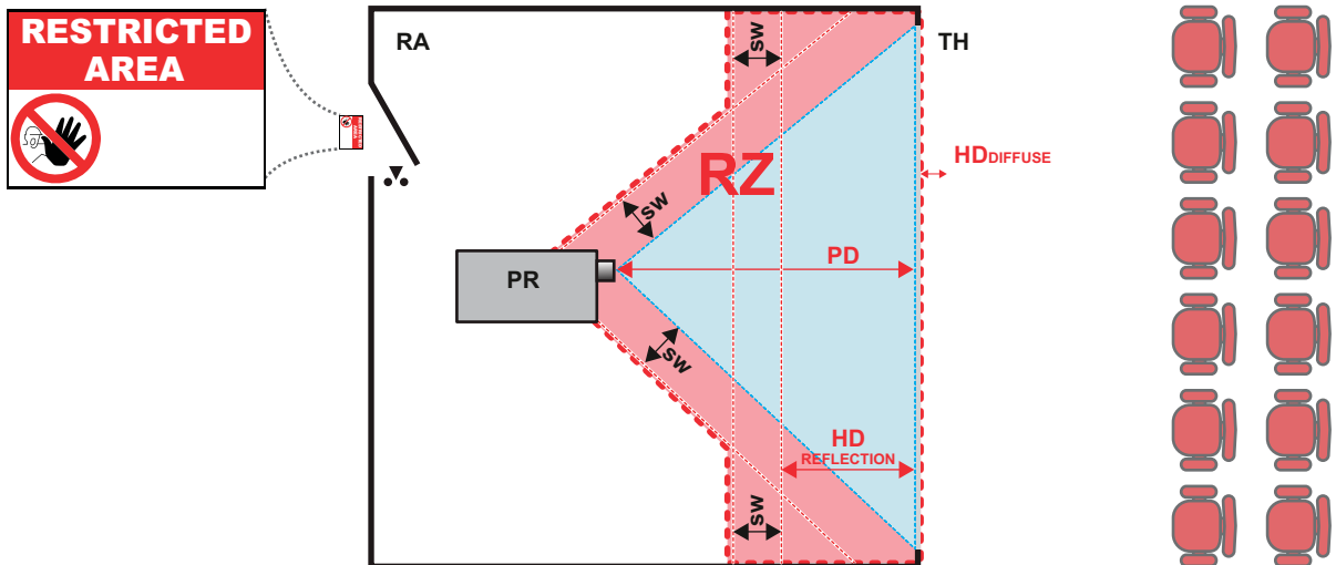
Image 1-3 RA Restricted Access location (enclosed projection area). PR Projector. TH Theater (observation area). RZ Restriction Zone. PD Projection Distance. SW Separation Width. Must be minimum 1 meter.
