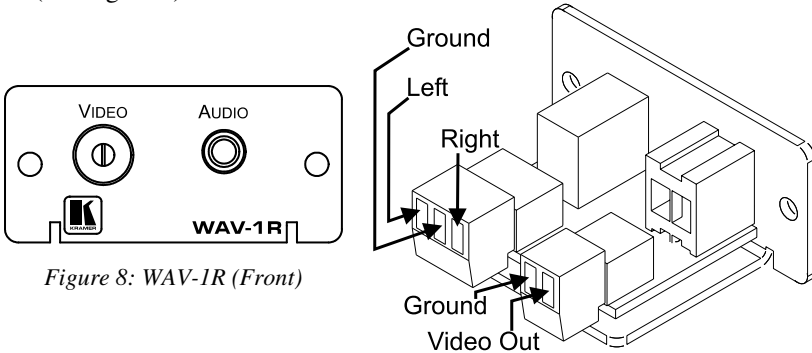
Figure 9: WAV-1R (Rear)
