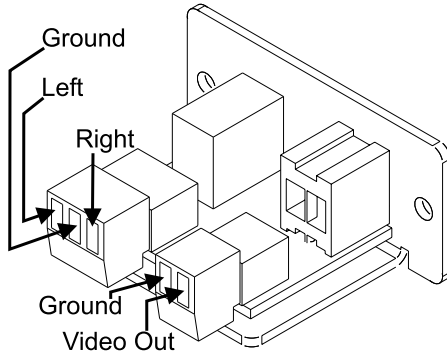
Figure 9: WAV-1R (Rear)
