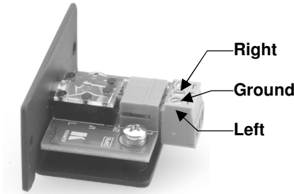
Figure 7: WA-1H (Rear)
