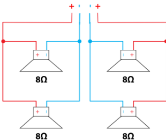
Example showing four 8Ω speakers
