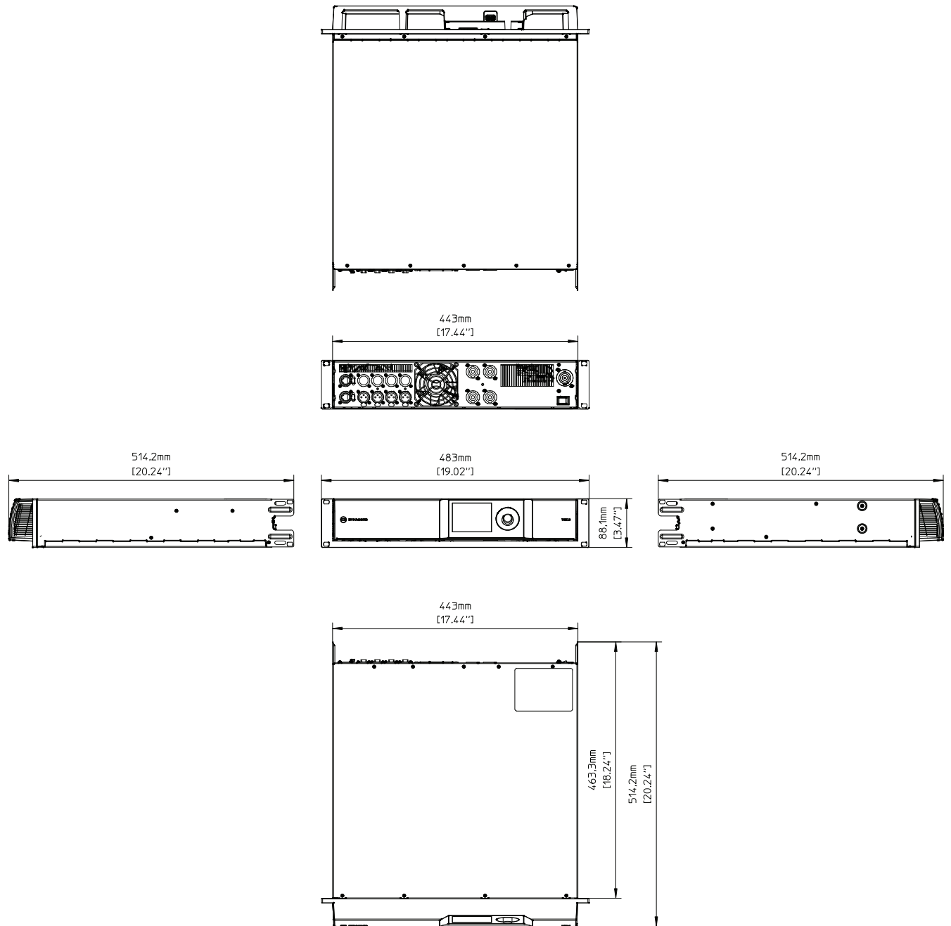
Figure 8.2: Dimensions: TGX
