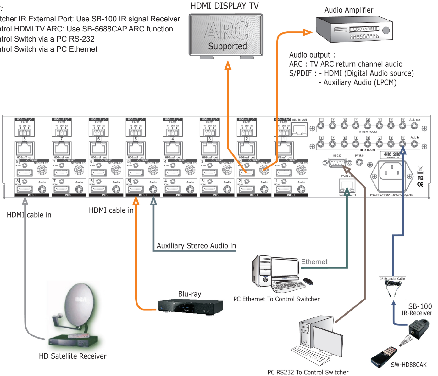
The RS-232 application, IR and Ethernet control the switcher.
