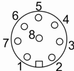
Figure 13- M12 Connector Wiring Method
