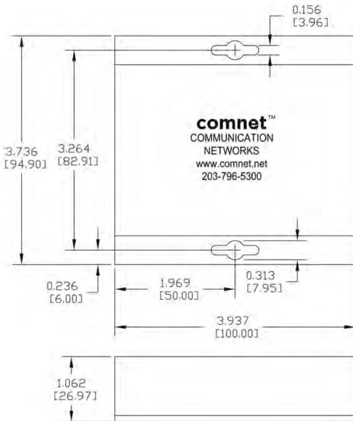
Figure 1: Dimensions are for a ComNet™ surface mount unit.
