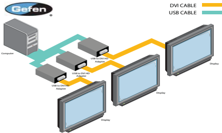
Figure 1: Adding Several Adapters/Displays to one PC
