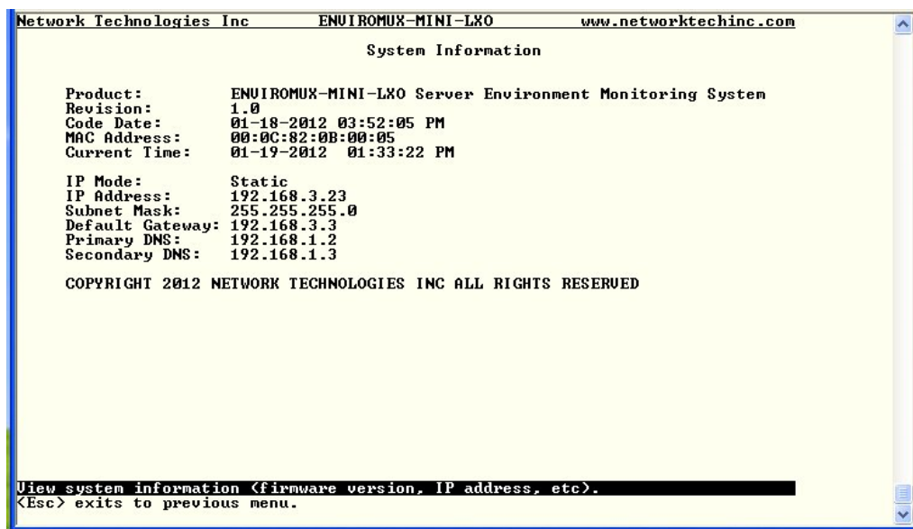
Figure 118-Text Menu-System Information
