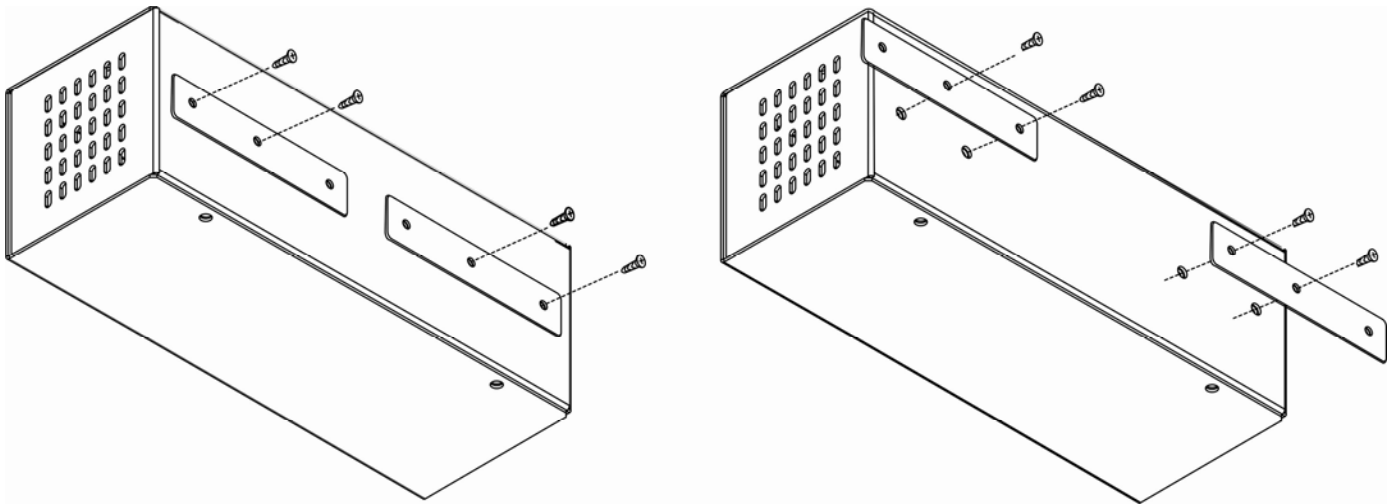
Figure 1- Rotate the tabs for Zero-RU mounting
