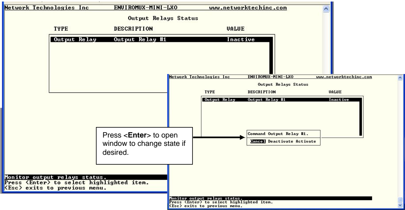
Figure 72- Text Menu- View Output Relay Status
