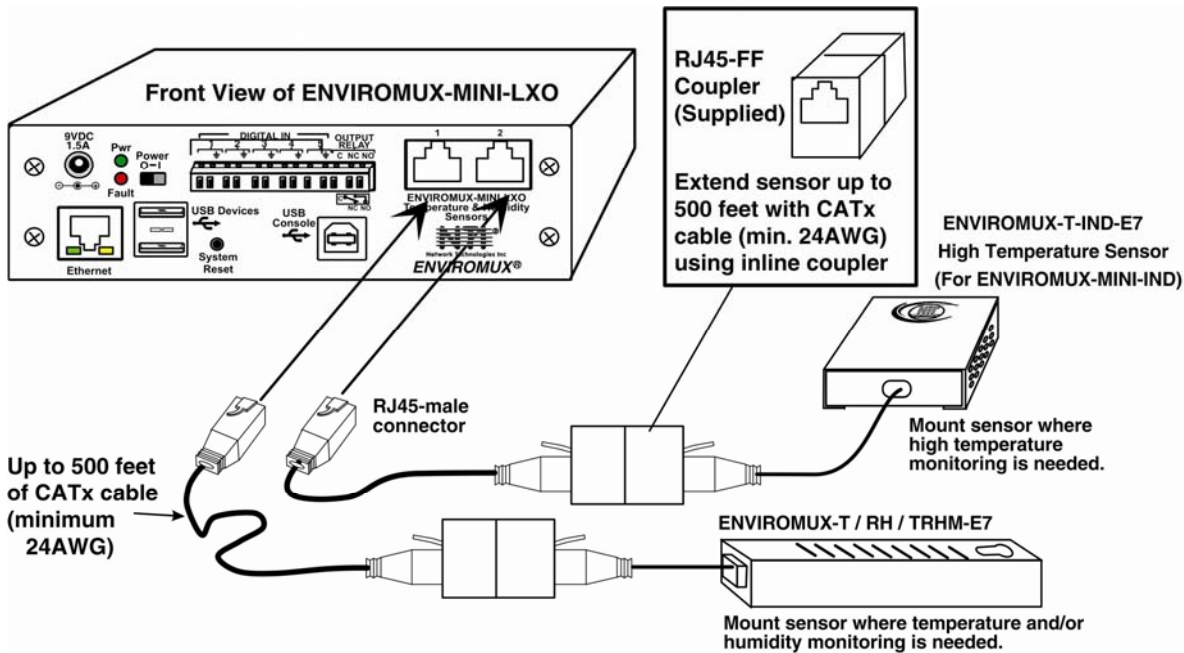
Figure 3- Connect Sensors
