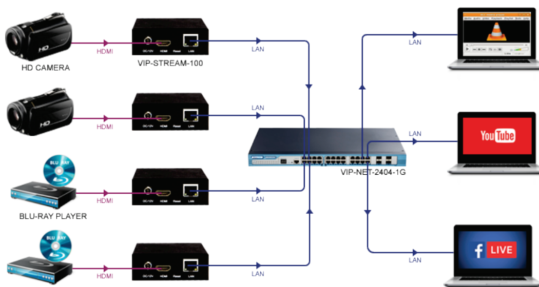
Multiple HDMI Sources to PC/Decoding Software over IP Network
