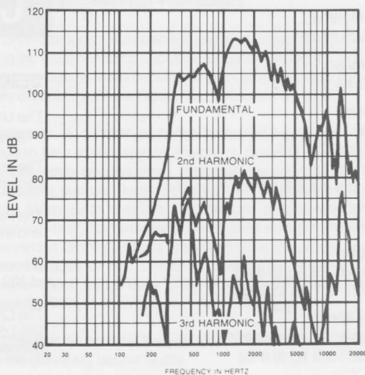
FIGURE 3 CFID32 Frequency Response (1 watt at 1 meter)
