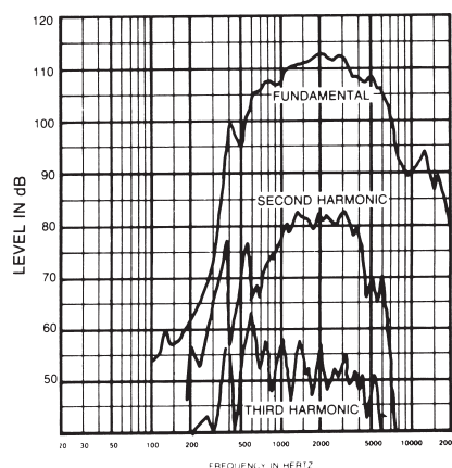
Figure 3 PA60 Frequency Response (1 watt at 1 meter)
