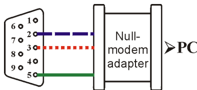
Figure 7: Straight Cable RS-232 Connection with a Null Modem Adapter
