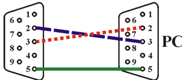
Figure 6: Crossed Cable RS-232 Connection
