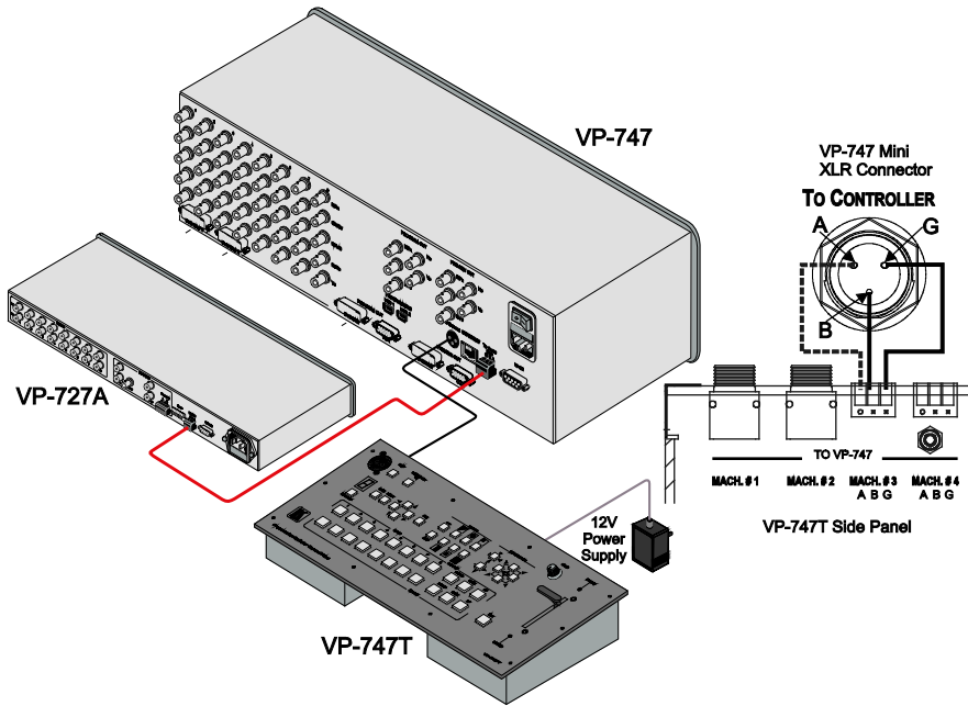
Figure 9: Connecting the VP-747 to the VP-747T
