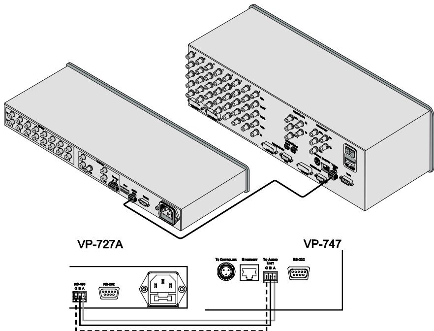
Figure 8: Connecting the VP-727A to the VP-747
