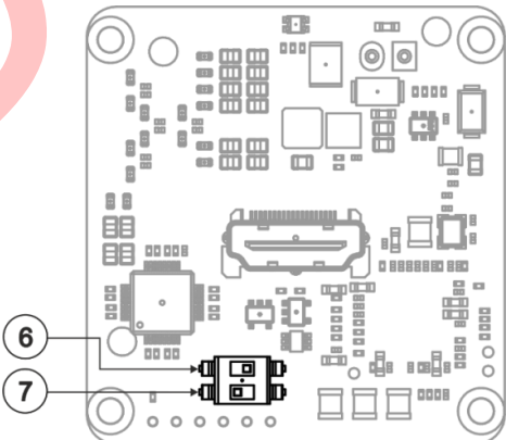
Figure 6: WP-871xr Line Transmitter Wall-plate – Behind the Front Panel
