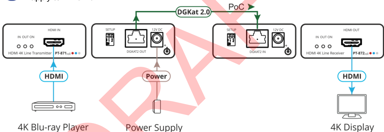
Figure 7: Connecting to PT-871/2xr-KIT
