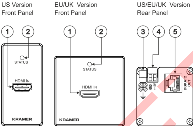
Figure 5: WP-871xr Line Transmitter Wall-plate
