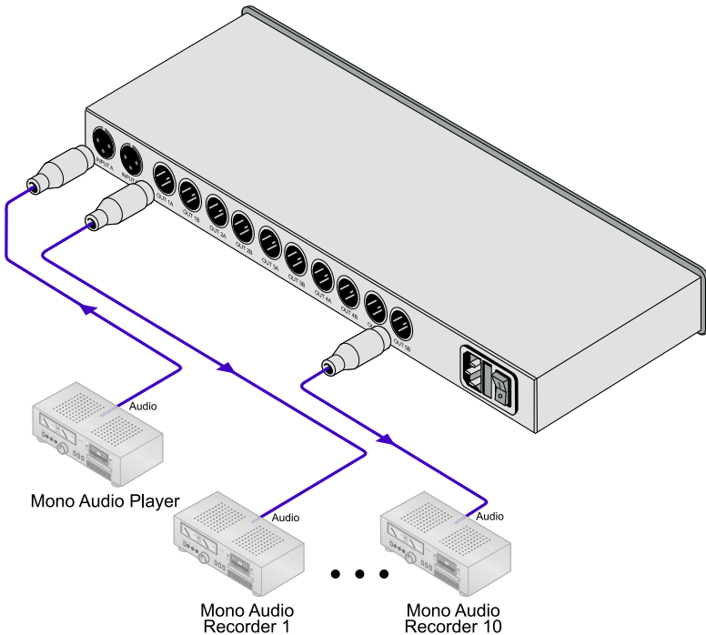
Figure 2: Connecting the VM-1110xl as a 1:10 Mono DA
